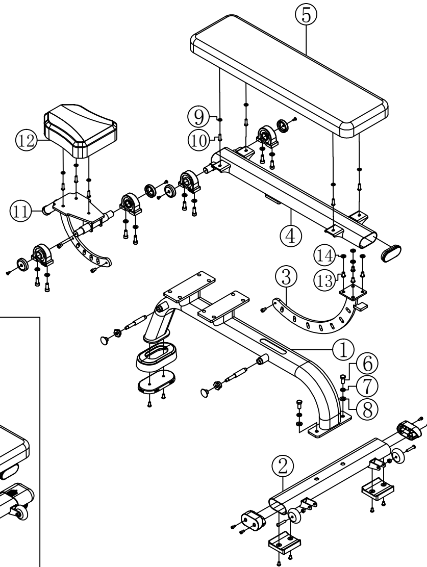
FF39 Adjustable bench explosive view
